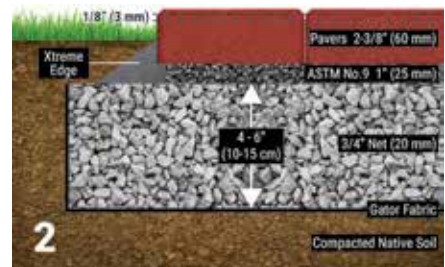
Option 2 • Open graded / Permeable
